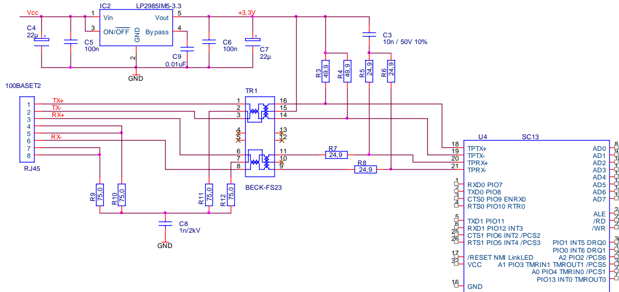
picture 10.7: Example of connecting 10/100Base-T to SC13 with FS23
